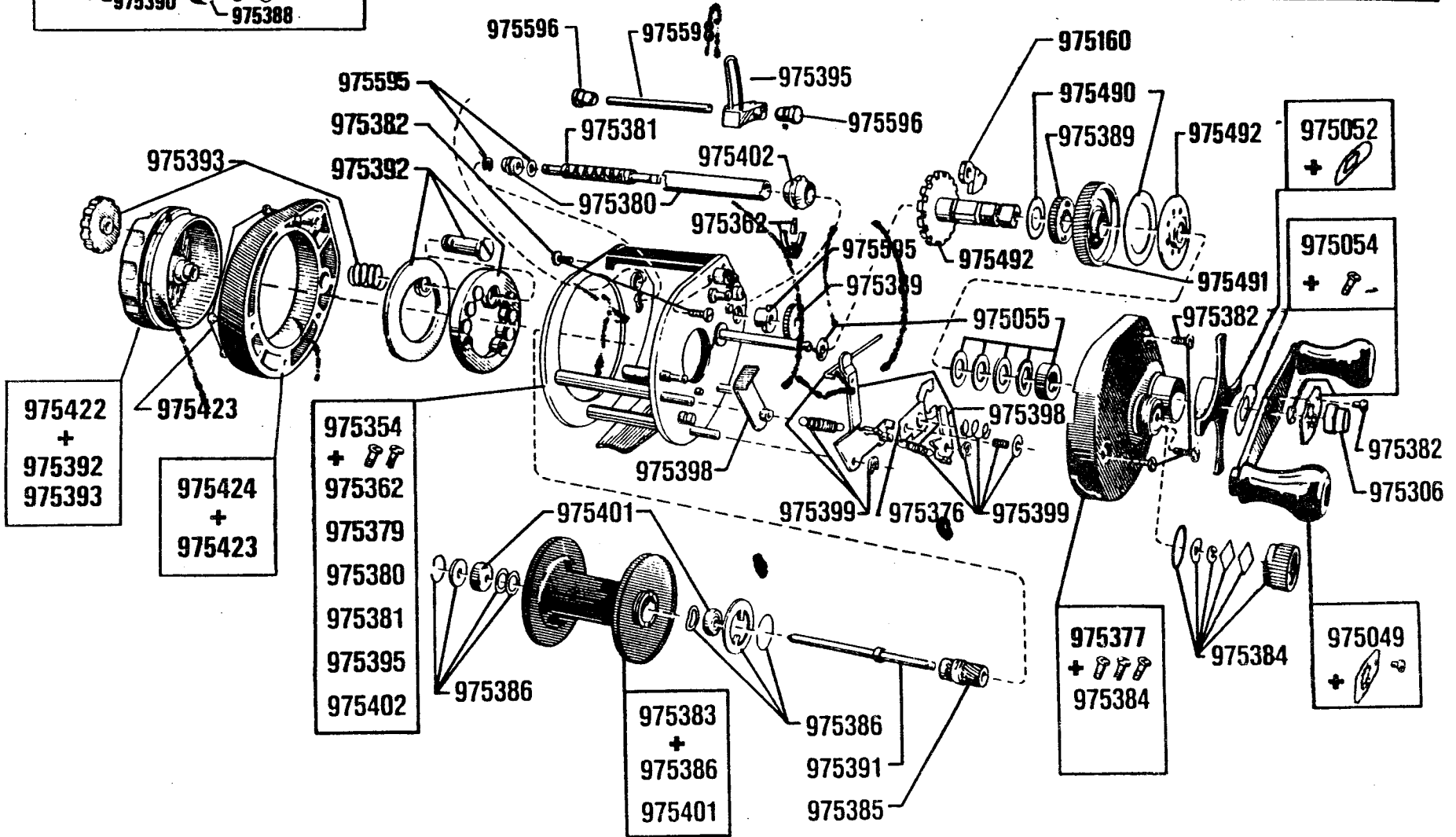
Ambassadeur ULTRA MAG XL II 83-2
